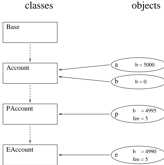
Figure 3: Inheritance hierarchy
