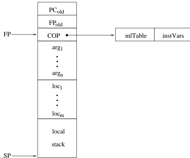
Figure 5: Stack frame
